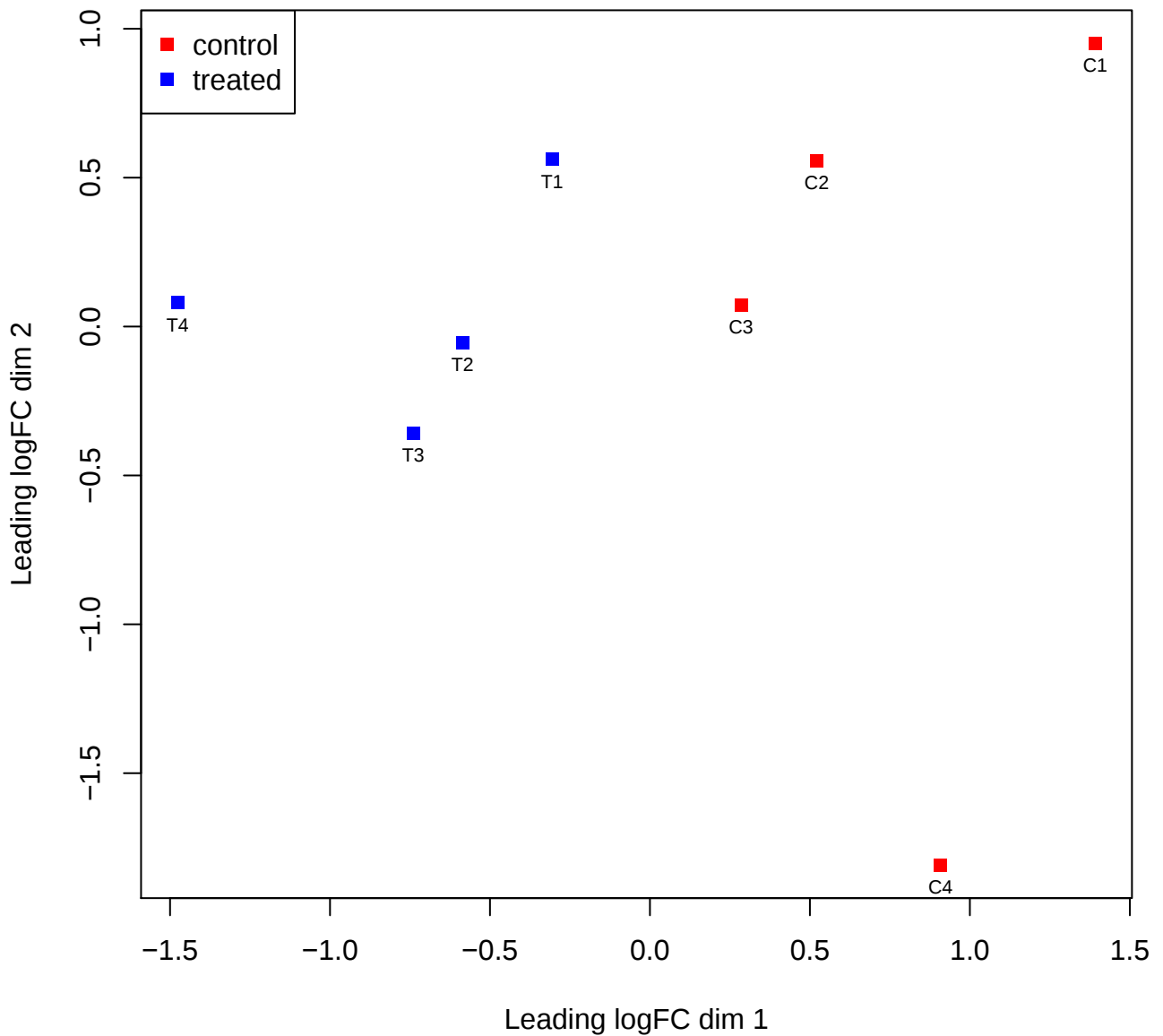
MDS Plot
