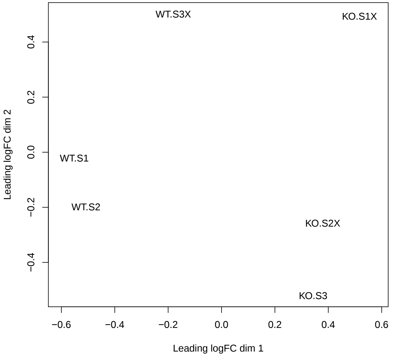
MDS Plot
