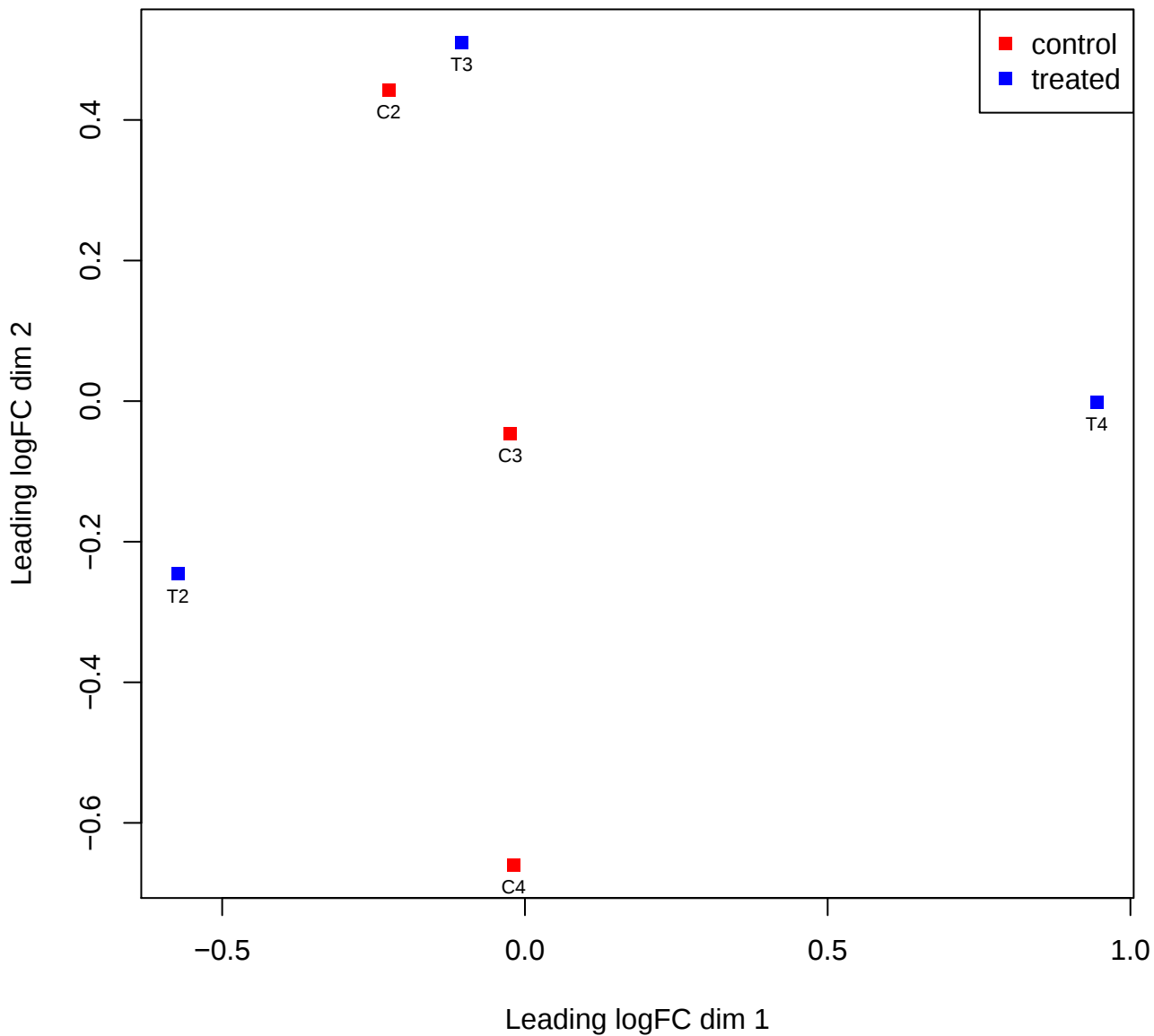
MDS Plot
