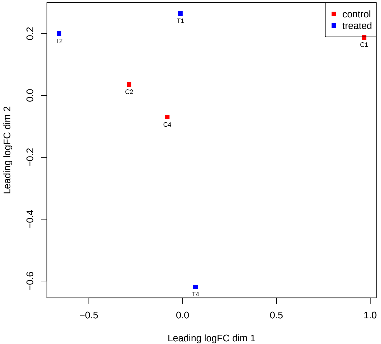
MDS Plot
