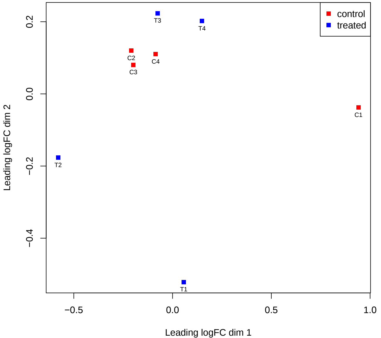
MDS Plot
